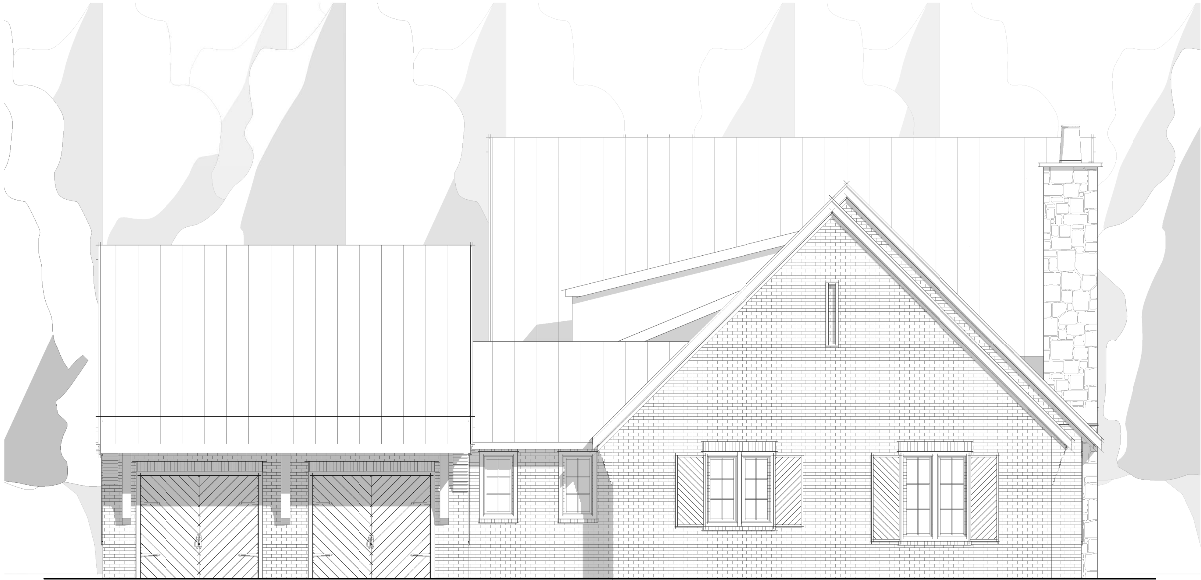
1 LEFT ELEVATION 1/4" = 1'-0"
