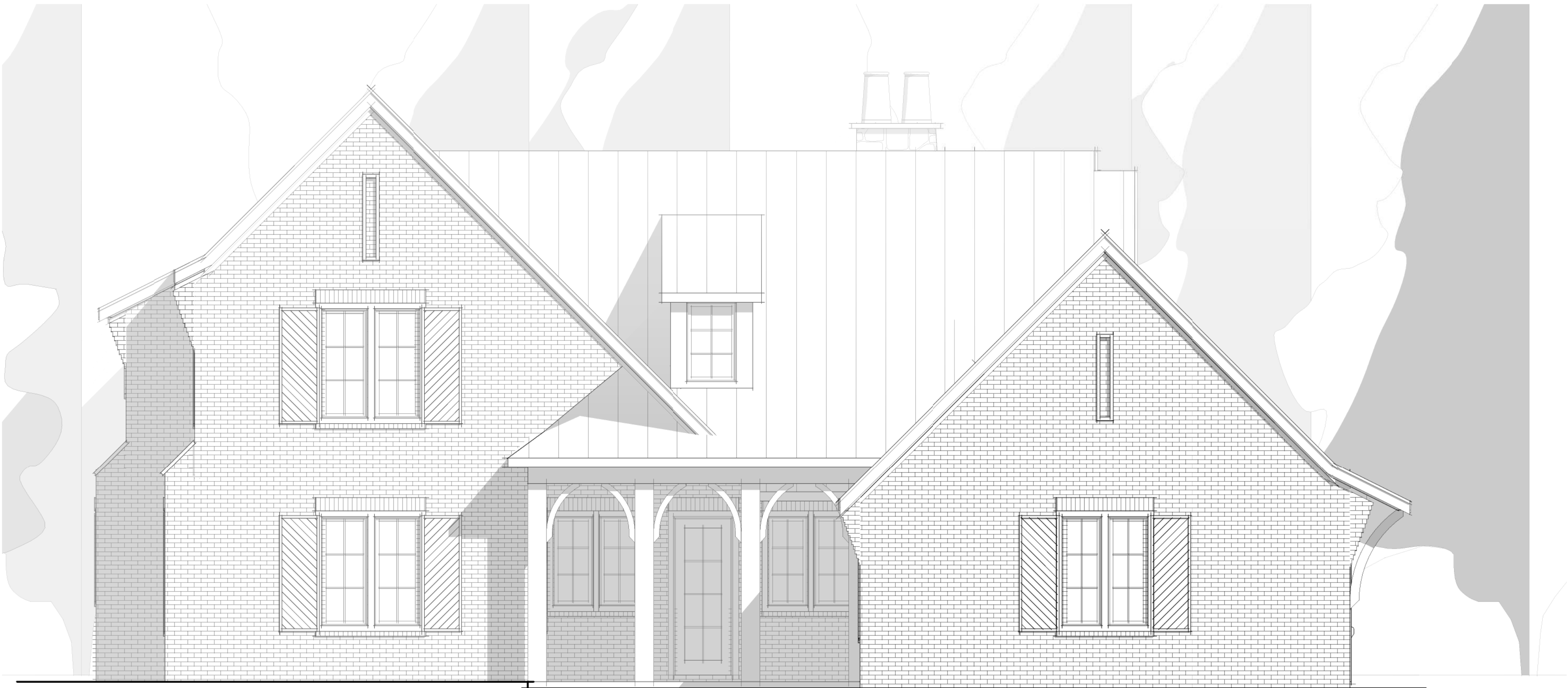
1 REAR ELEVATION 1/4" = 1'-0"
